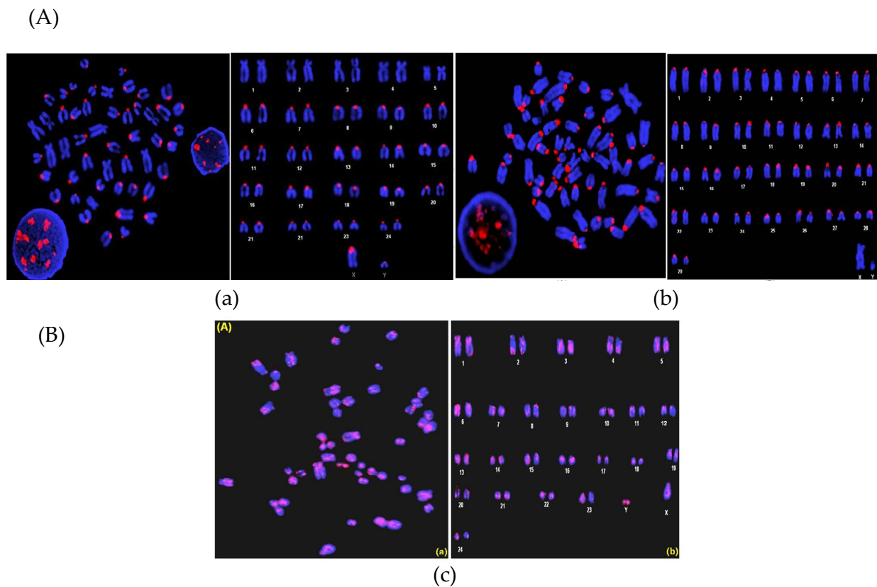
Figure 6. Chromosomal localization of pDS5 clone (A) on (a) buffalo and (b) cattle metaphase chromosomes. Note the absence of signal in all the bi-armed chromosomes. Fluorescence in situ hybridization (FISH) of pDp1 (B) clone on buffalo metaphase chromosomes (c). Note the dispersed signals over the metaphase chromosomes. (See Pathak et al 2006; 2011).
